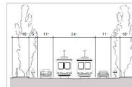
Figure 22: Typical Girard Road Section
